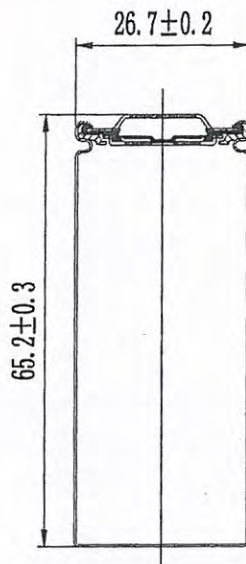
图1 电芯外观尺寸 Figure 1 Cell appearance size
